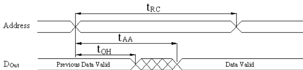
READ CYCLE 1. (1, 2, 4)
