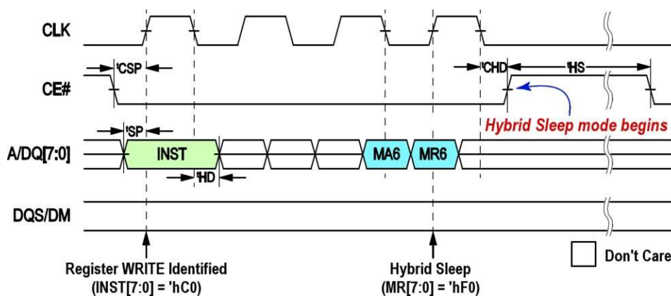
Figure 14: Hybrid Sleep Entry Write (default WL0)
