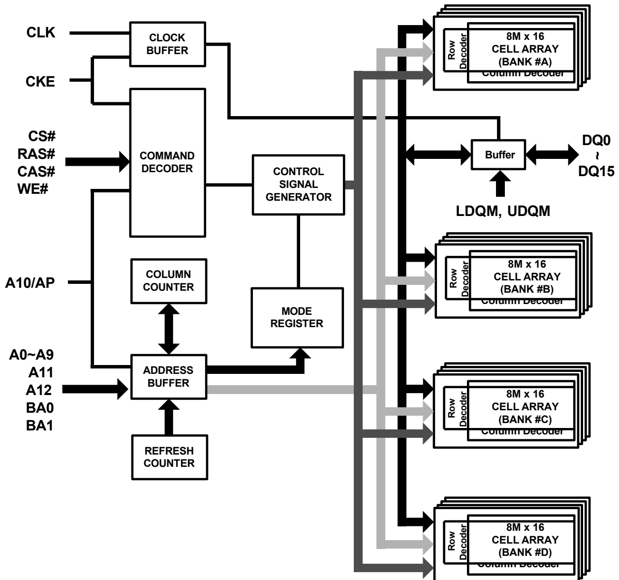
Figure 2. Block Diagram
